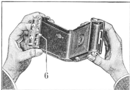
Fig. 10. Opening the film-chamber
