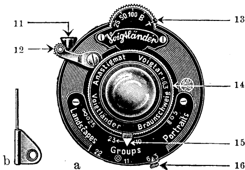
Fig. 3. Shutter, with three-point focussing
