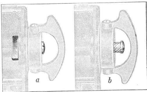
Fig. 12. Film winding-key
